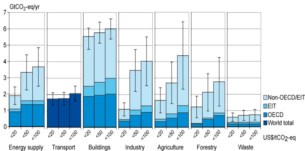
Estimated economic mitigation potential by sector and region using technologies and practices expected to be available in 2030. The potentials do not include non-technical options such as lifestyle changes. Source: IPCC, 2007 4 .
